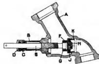
Fig. 3172. Section of End Train Pipe Valve, No. 200.
